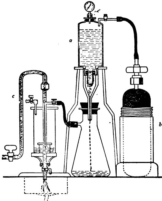
FIG. 38.—Pakes' filtering reservoir—pressure and aspiration.
